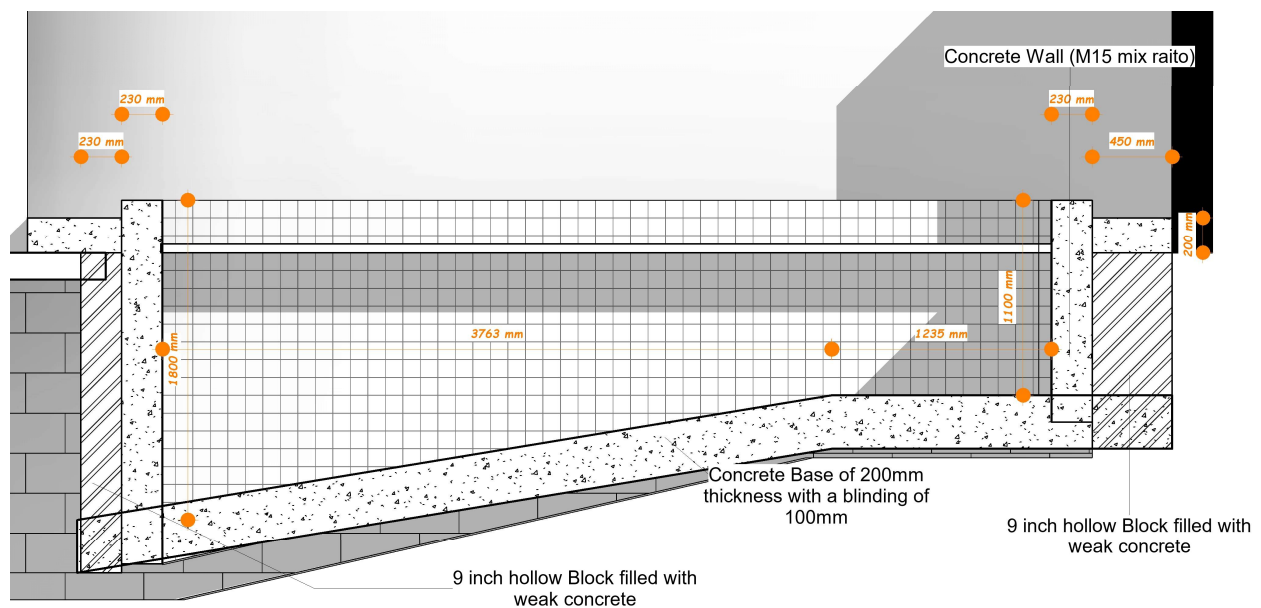
Fig. 2 — Longitudinal Section A — Detail (DWG A-02) · All dimensions in millimetres
