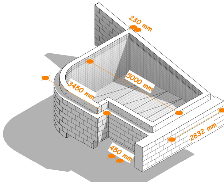
Fig. 4 — Rear-Left View (DWG 3D-02) · Curved wall & coping detail
