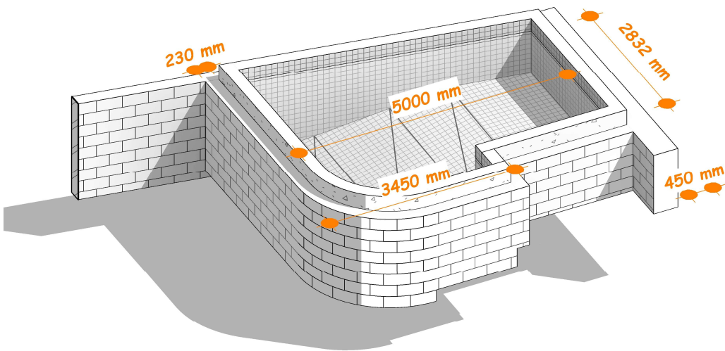
Hotel Swimming Pool — 3D Axonometric View
