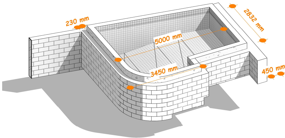
Fig. 3 — 3D Axonometric: Front-Right View (DWG 3D-01) · Showing external blockwork.
