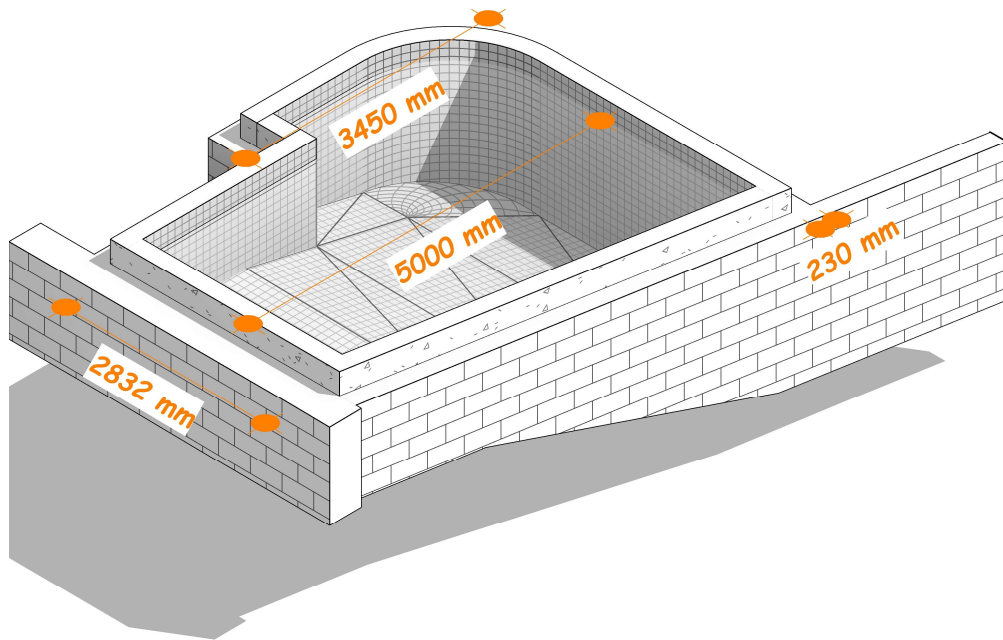
Fig. 5 — Interior View (DWG 3D-03) · Sloped floor, step pit & wall section
